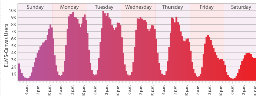
ELMS-Canvas usage distribution during a week of the Spring 2017 semester (April 16-22, 2017).
